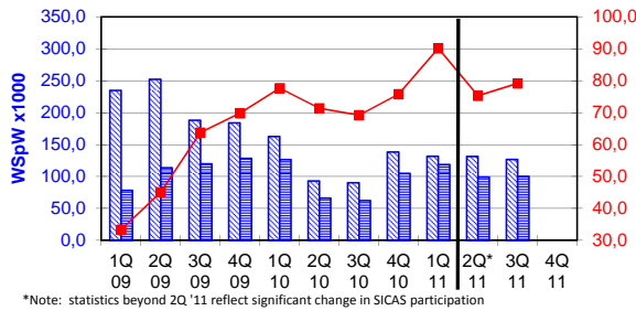
300mm Wafers in MOS Total
